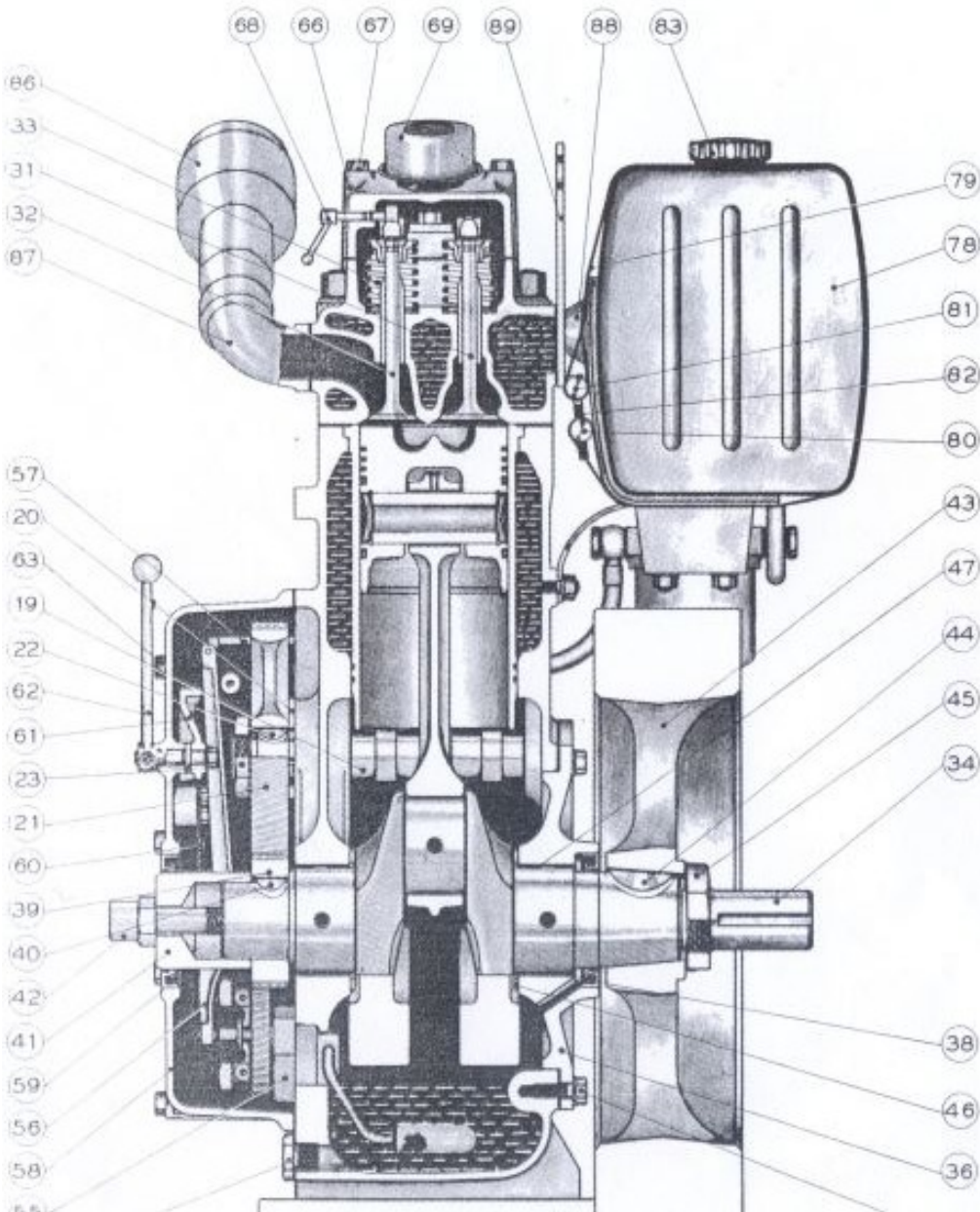
SUPER STAR DIESEL ONE CYLINDER ENGINE CROSS-SECTION A
